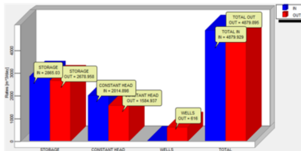
Scenario 3 – PUMPING 50% mine requirement =616 m 3 /day – Mass balances
